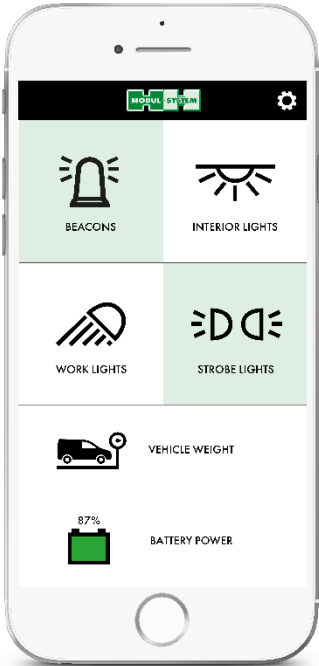
Manage lights
